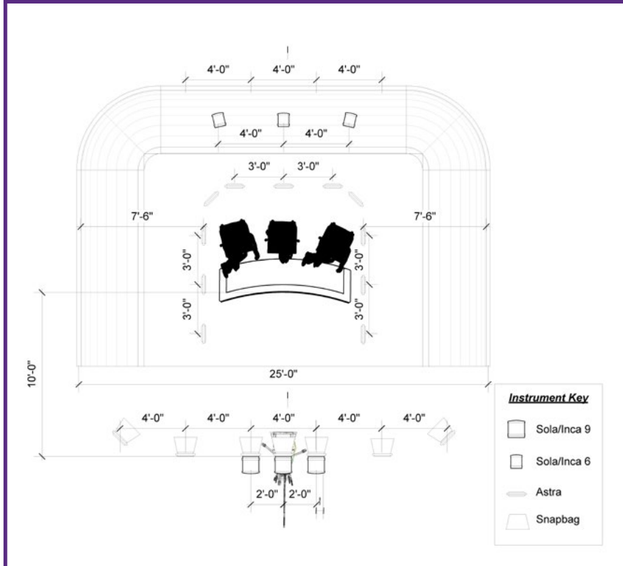
PLAN VIEW
